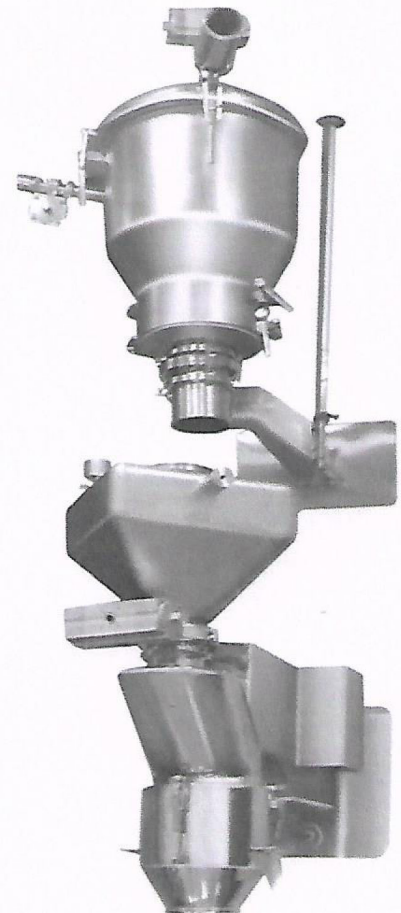
POWDER TRANSFER SYSTEM (JAY PHARMA PTS)
